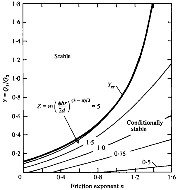
FIGURE 6. Stability diagram based on (20) and (21) which illustrates the relationship between the heating ratio Y = Q_1/Q_2 , the friction exponent n (from (4)), and the parameter Z . Y -values above and below Y_{cr} correspond, respectively, to stable and conditionally stable flows. For Y < Y_{cr} , flows are stable provided Z is less than the critical value shown on the curves.
